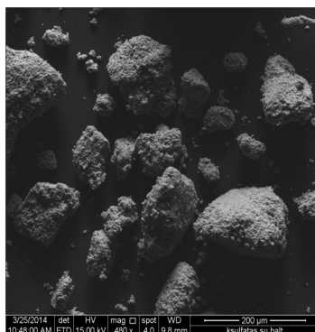
Fig. 1. Scanning electron micrographs: a – K 2 SO 4 raw crystals, b – RML PCMC
